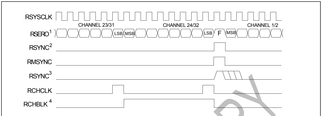
Figure 12-22 Receive-Side Boundary Timing, RSYCLK = 1.544MHz (E-Store Enabled)
