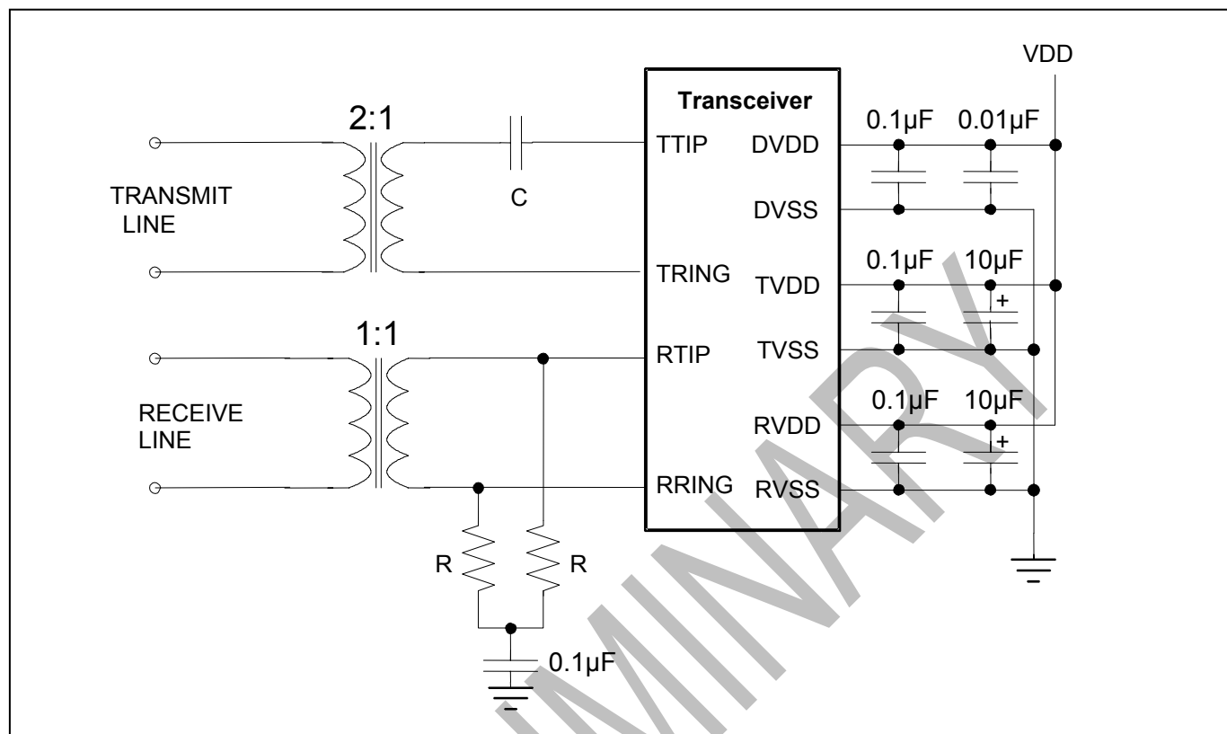
Figure 10-7 Basic Interface
