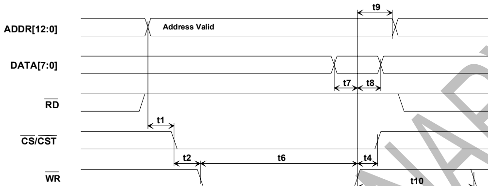
Figure 13-10 Intel Bus Write Timing (MODEC = 00)
