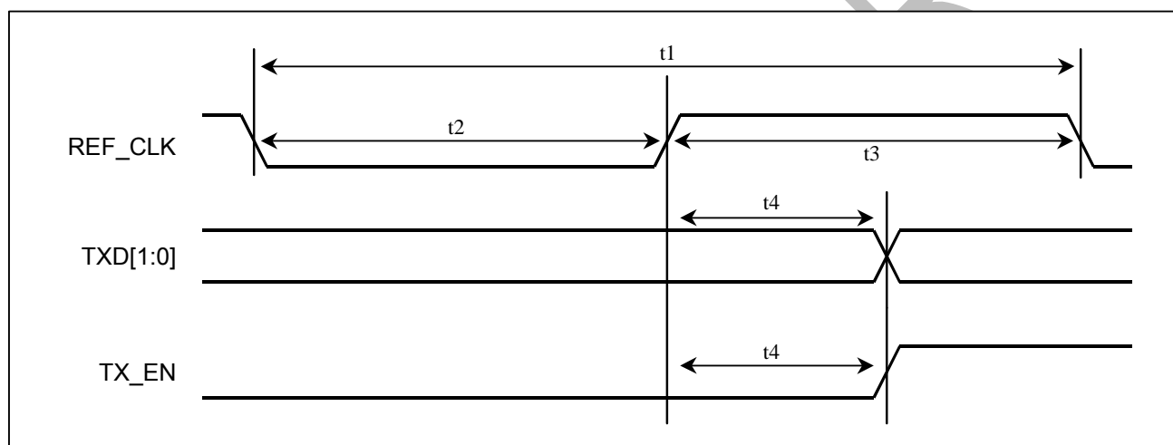
Figure 13-3 Transmit RMI Interface
