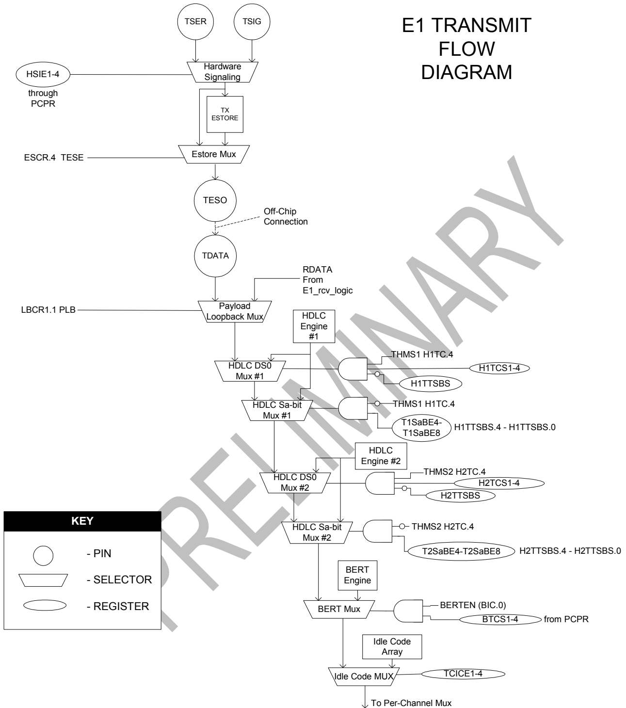
Figure 10-18 E1 Transmit Flow Diagram
