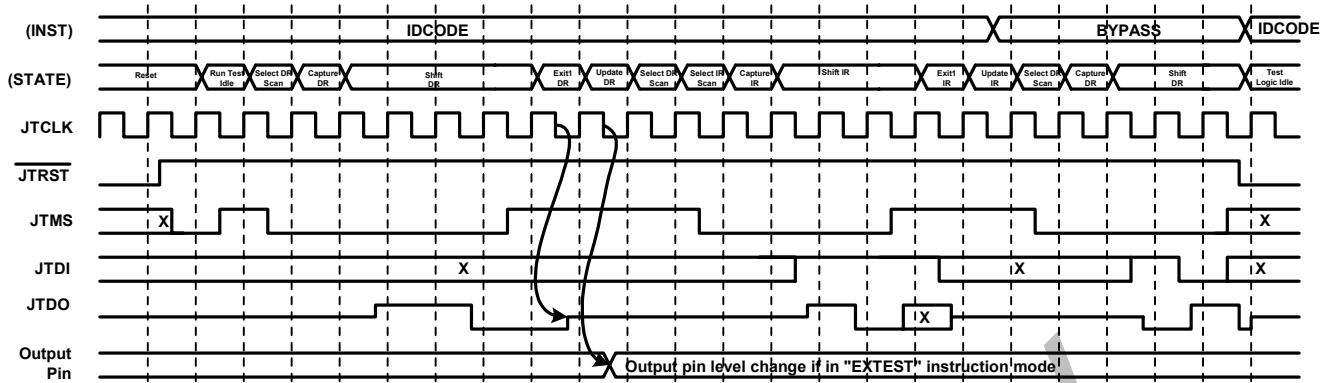
Figure 14-3 JTAG Functional Timing
