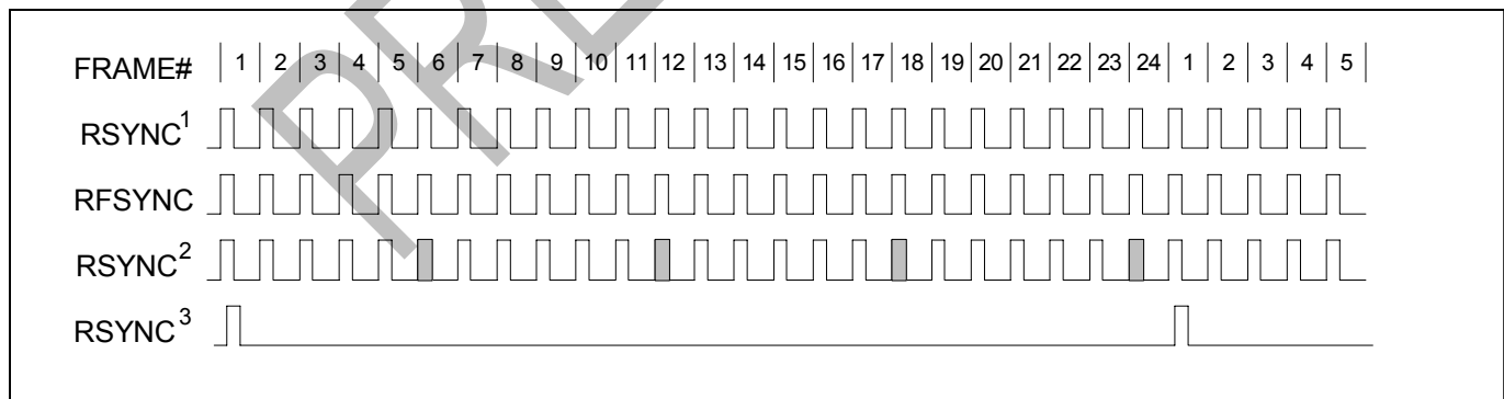
Figure 12-11 Receive-Side ESF Timing
