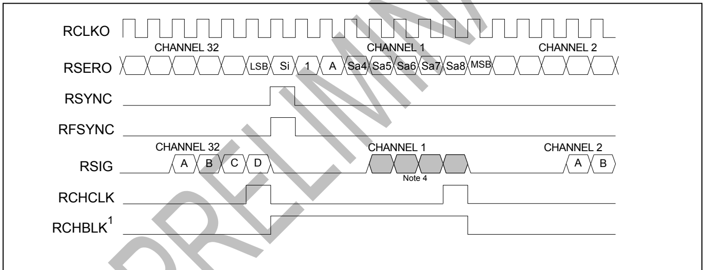
Figure 12-21 Receive-Side Boundary Timing (with Elastic Store Disabled)
