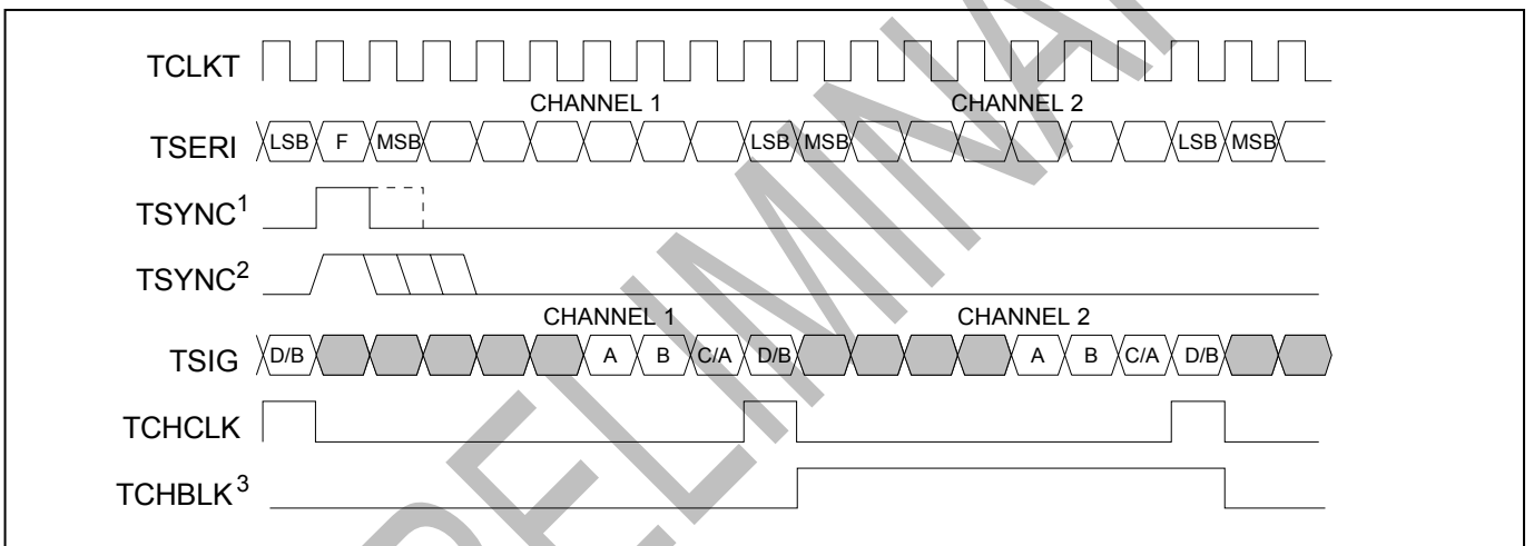
Figure 12-17 Transmit-Side Boundary Timing (with Elastic Store Disabled)
