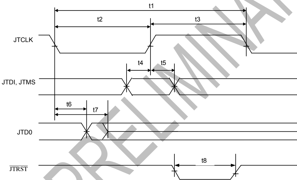
Figure 13-20 JTAG Interface Timing Diagram
