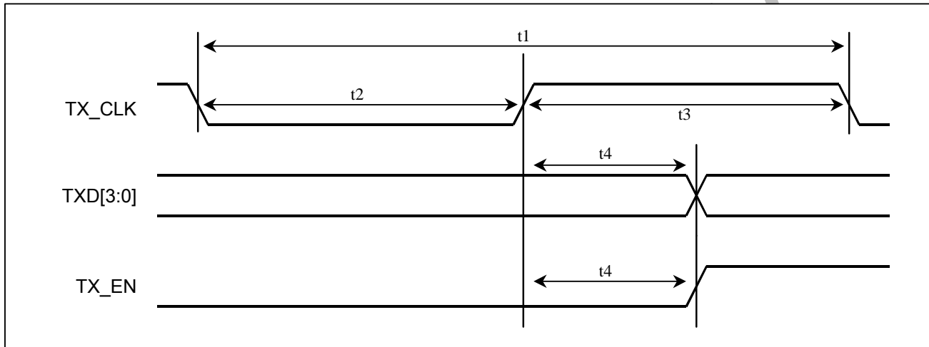
Figure 13-1 Transmit MII Interface
