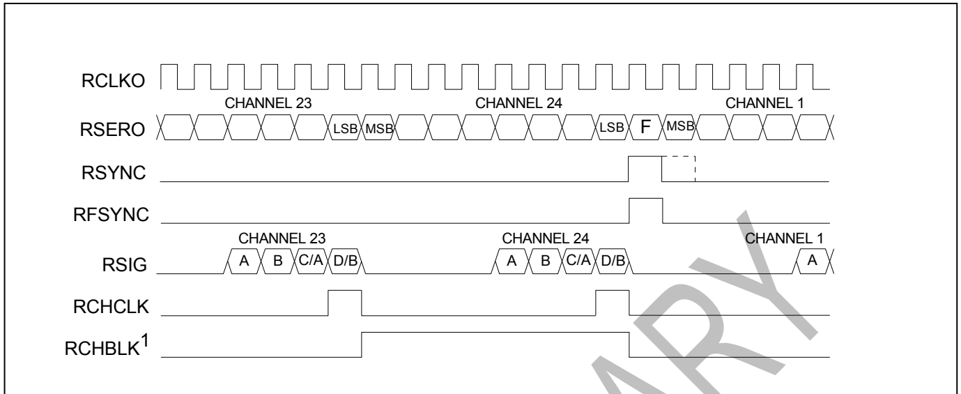
Figure 12-12 Receive-Side Boundary Timing (Elastic Store Disabled)
