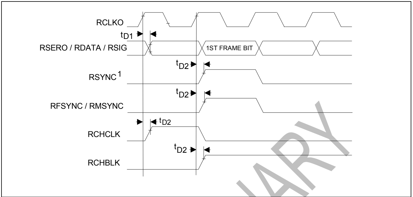
Figure 13-13 Receive-Side Timing
