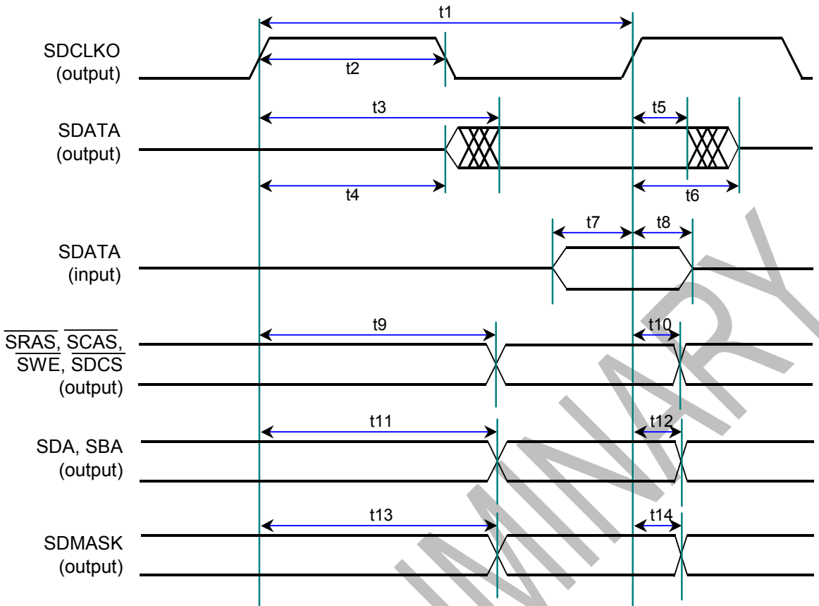
Figure 13-8 SDRAM Interface Timing
