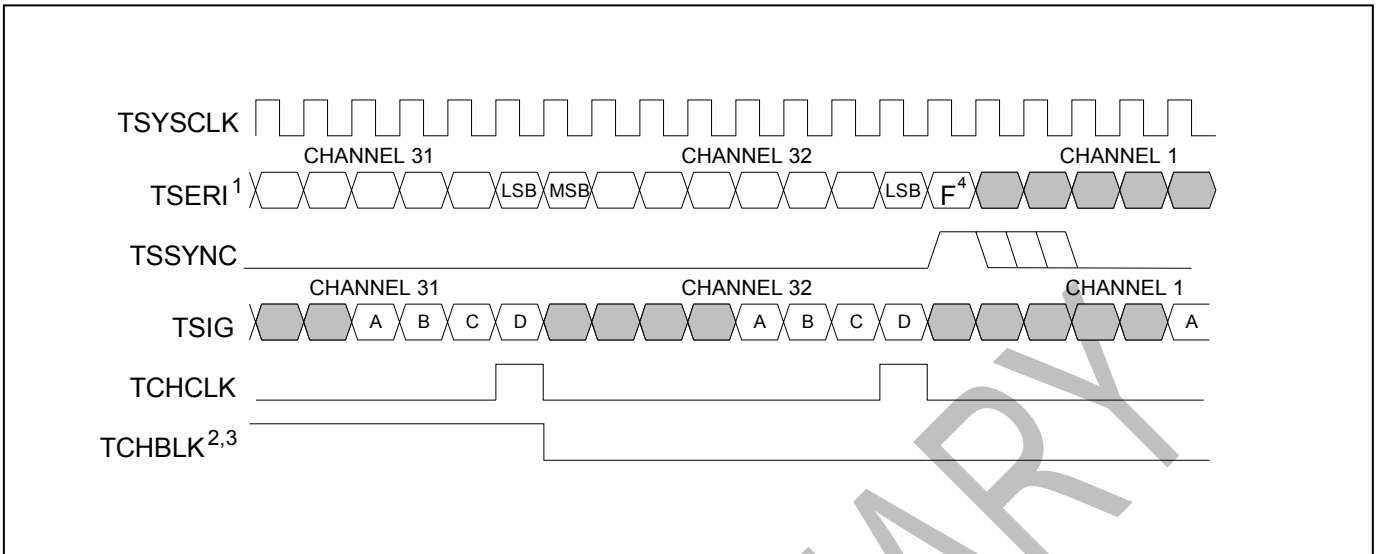
Figure 12-28 Transmit-Side Boundary Timing, TSYCLK = 2.048MHz (Elastic Store Enabled)
