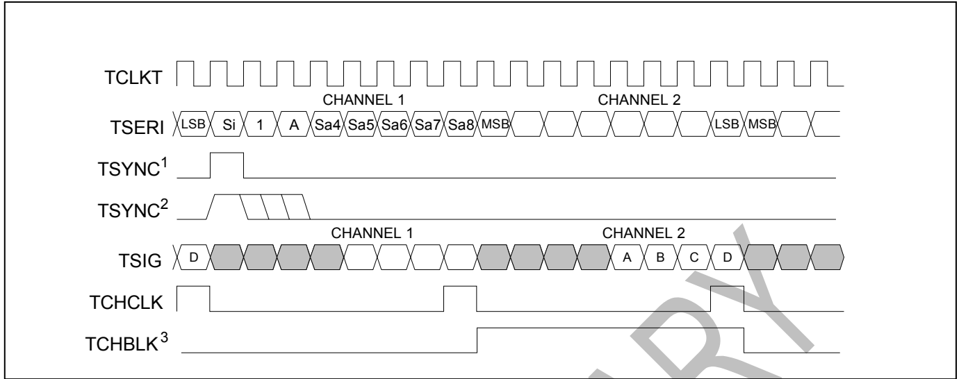
Figure 12-26 Transmit-Side Boundary Timing (Elastic Store Disabled)
