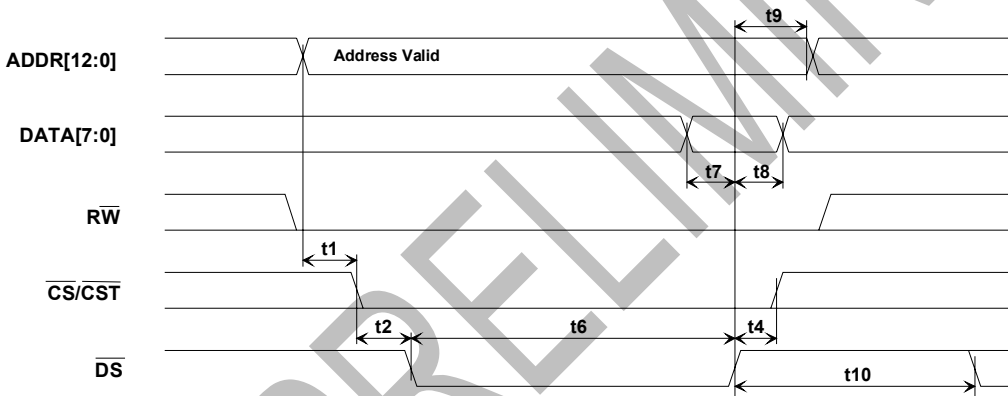
Figure 13-12 Motorola Bus Write Timing (MODEC = 01)
