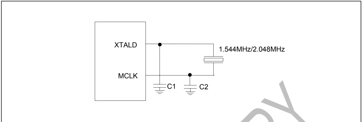
Figure 10-14 Optional Crystal Connections
