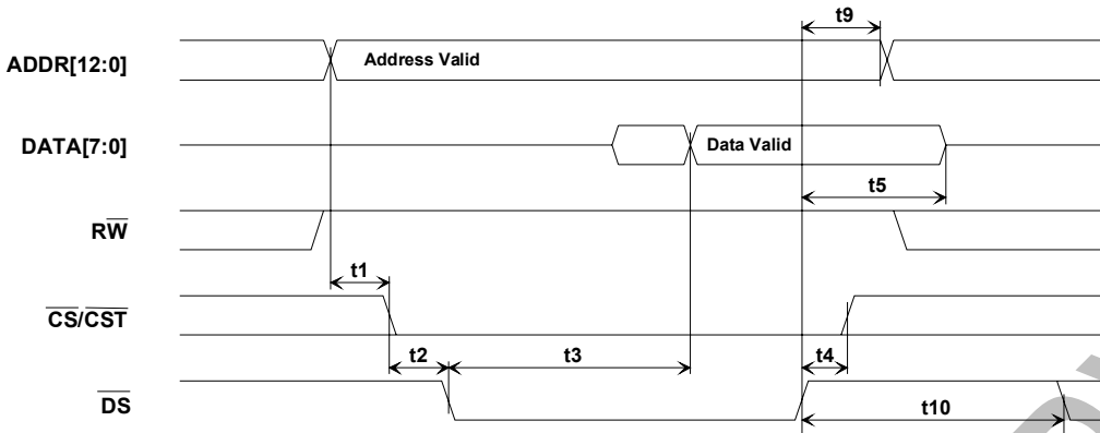
Figure 13-11 Motorola Bus Read Timing (MODEC = 01)
