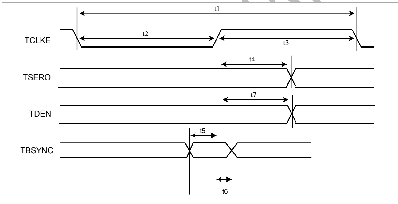
Figure 13-6 Transmit WAN Timing
