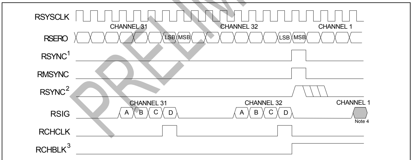
Figure 12-23 Receive-Side Boundary Timing, RSYCLK = 2.048MHz (E-Store Enabled)
