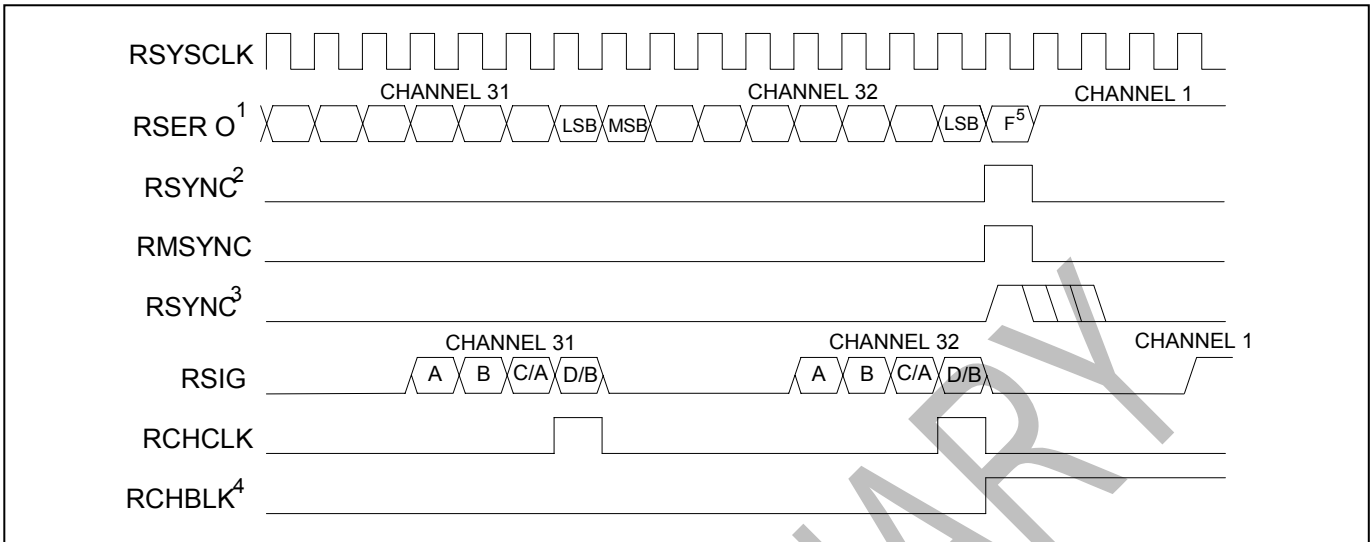
Figure 12-14 Receive-Side 2.048MHz Boundary Timing (Elastic Store Enabled)
