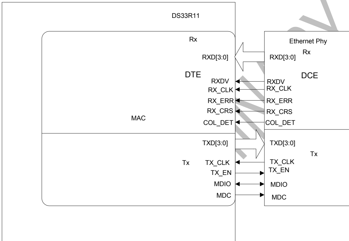
Figure 9-5 Configured as DTE connected to an Ethernet PHY in MII Mode
