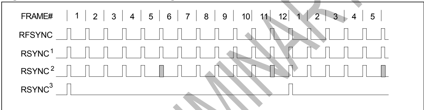
Figure 12-10 Receive-Side D4 Timing
