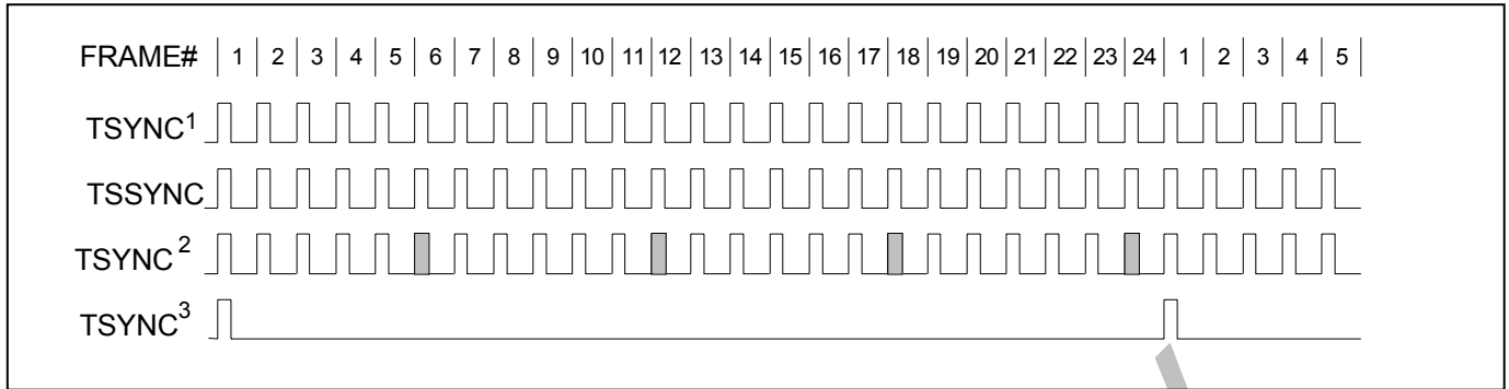
Figure 12-16 Transmit-Side ESF Timing
