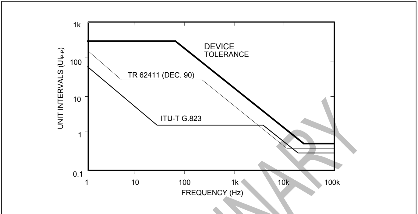
Figure 10-10 Jitter Tolerance
