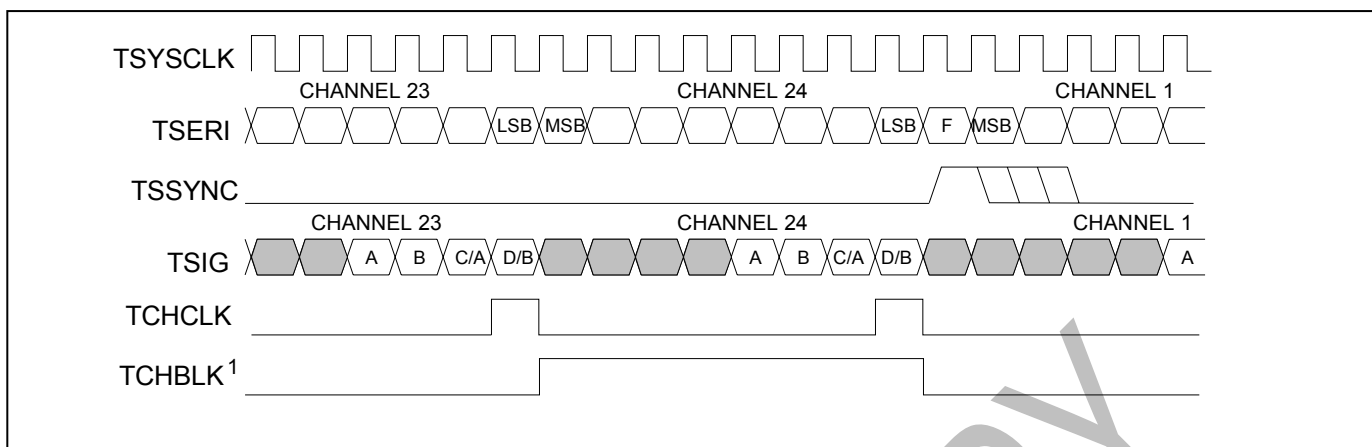
Figure 12-18 Transmit-Side 1.544MHz Boundary Timing (Elastic Store Enabled)
