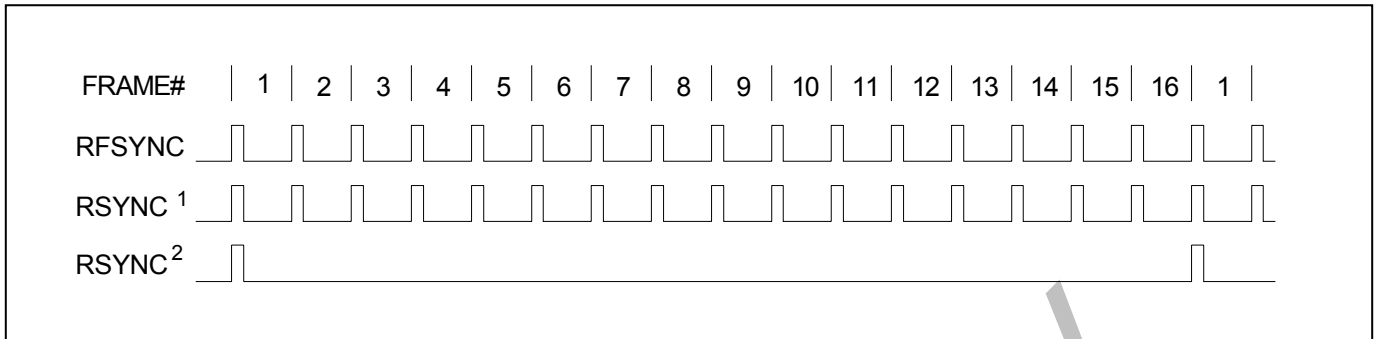
Figure 12-20 Receive-Side Timing
