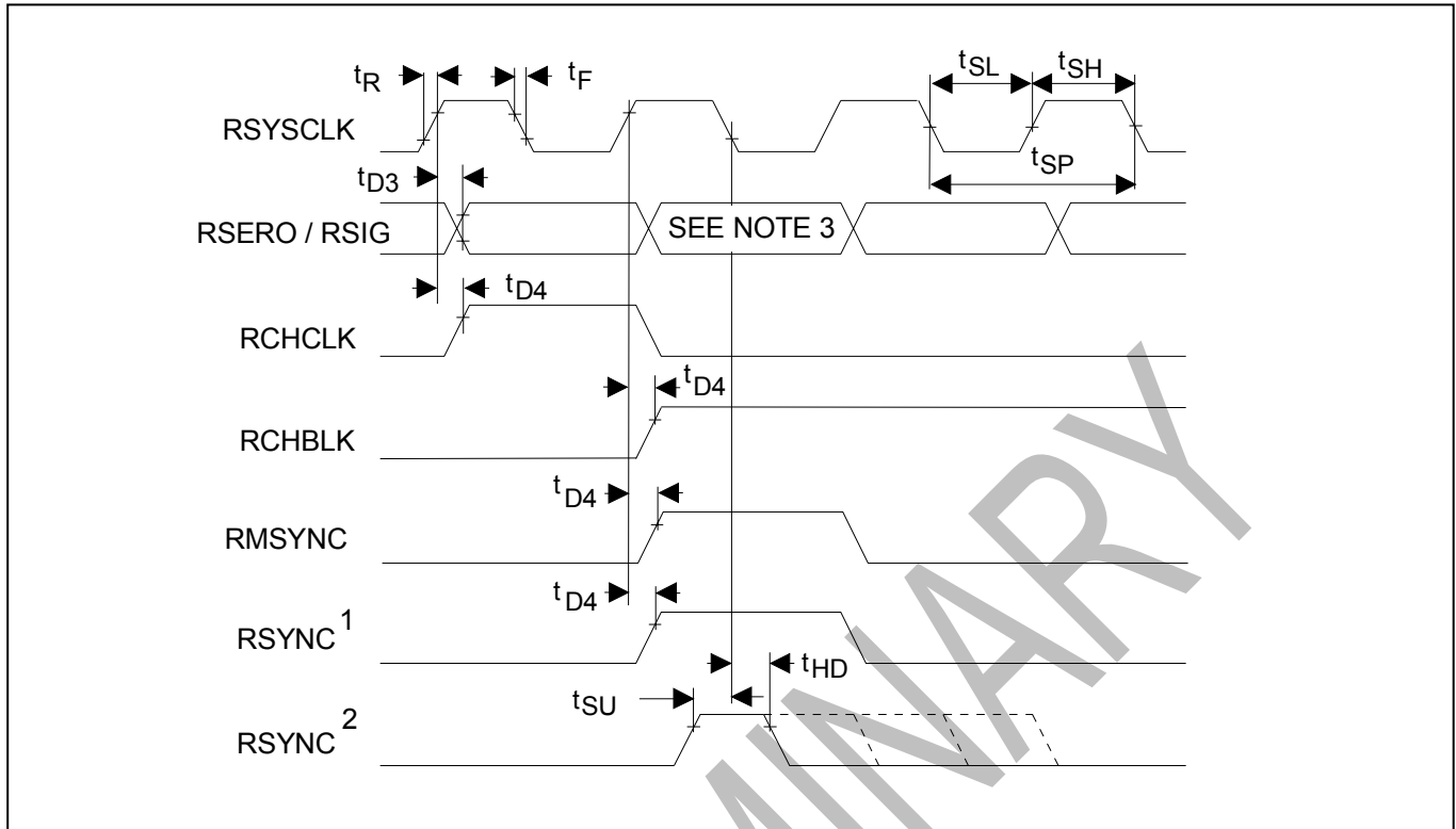
Figure 13-14 Receive-Side Timing, Elastic Store Enabled
