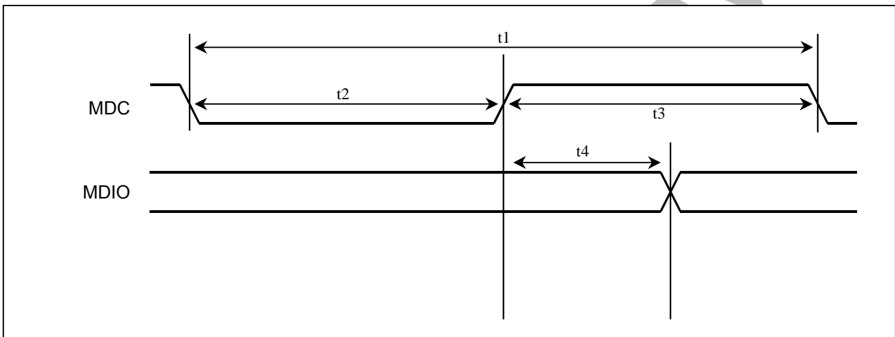
Figure 13-5 MDIO Timing
