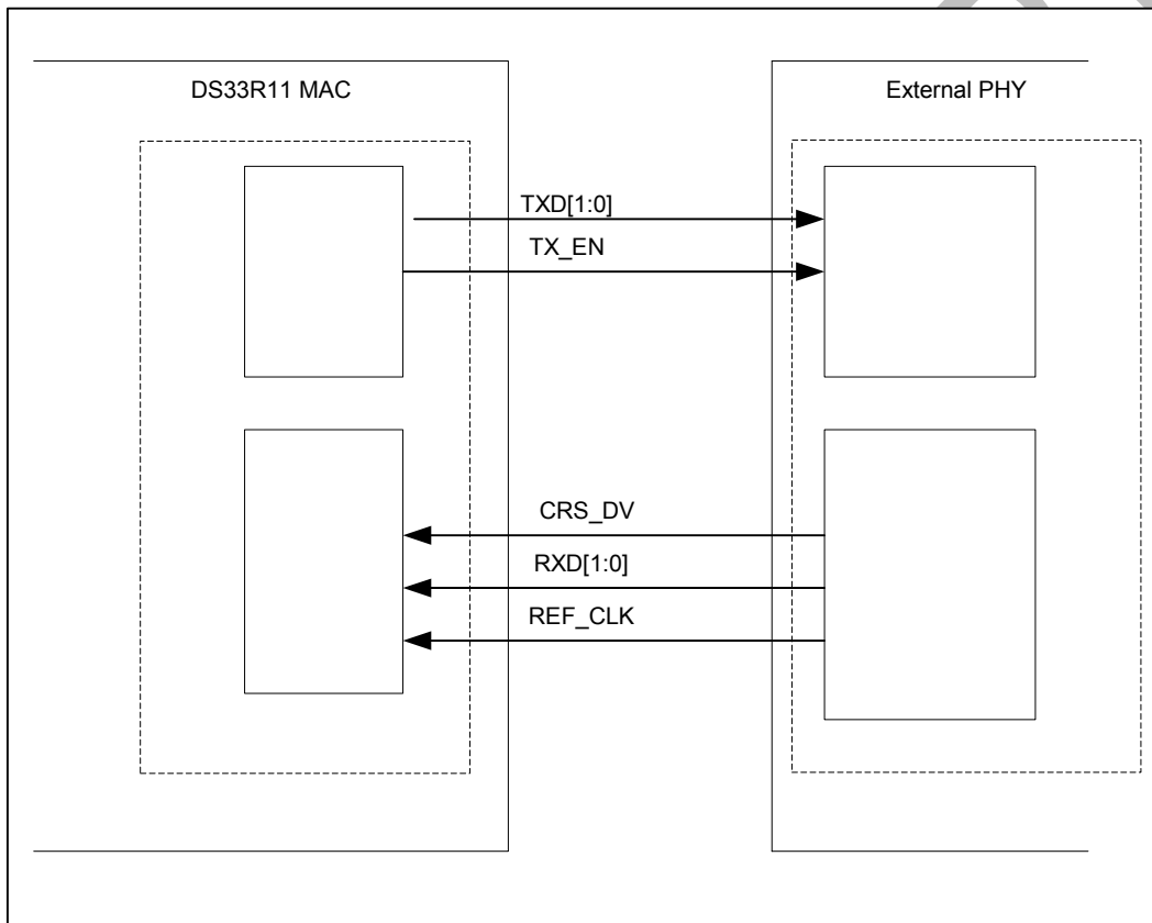
Figure 9-7 RMII Interface
