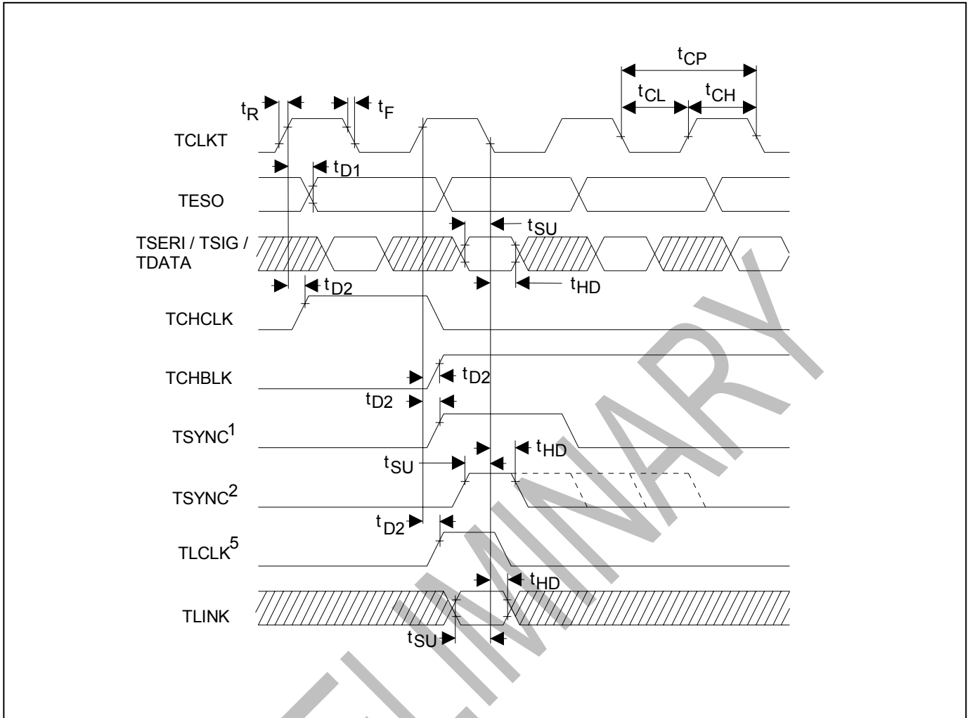
Figure 13-17 Transmit-Side Timing
