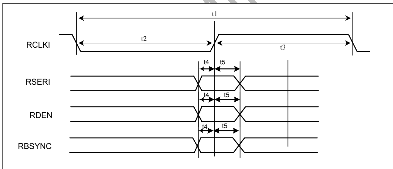
Figure 13-7 Receive WAN timing
